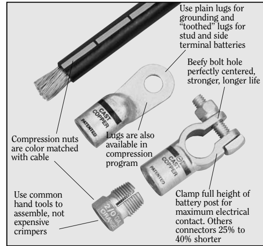
Compression battery connectors assemble with common hand tools
