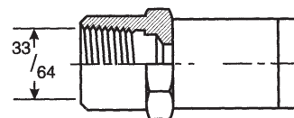
1/2-27 Tapered Thread (4-8FG)
